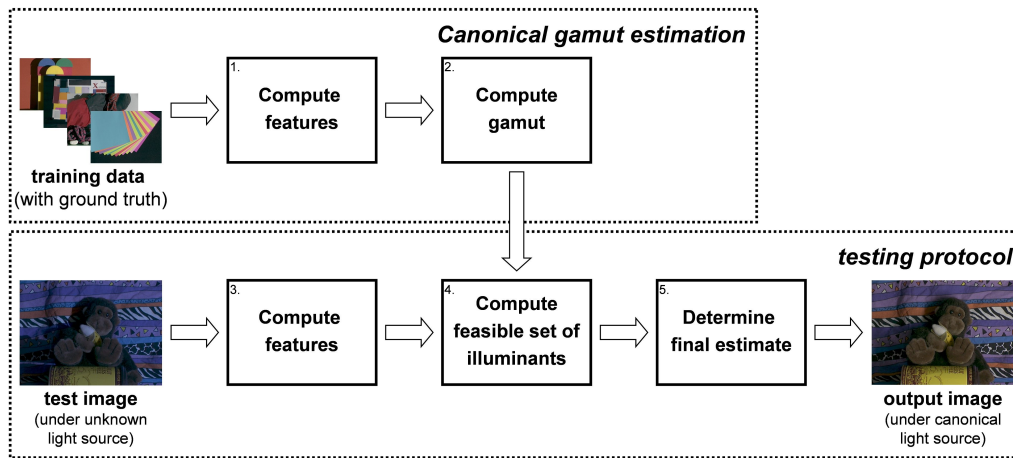
Fig. 2. Overview of gamut-based algorithms. The training phase consists of learning a model given the features of a wide variety of input images (block 1), resulting in the canonical gamut (block 2). The testing protocol consists of applying the learned model to the computed features of the input image (blocks 3 and 4). Finally, one illuminant estimate is selected from the feasible set of illuminants (block 5) and this estimate is used to correct the input image.
