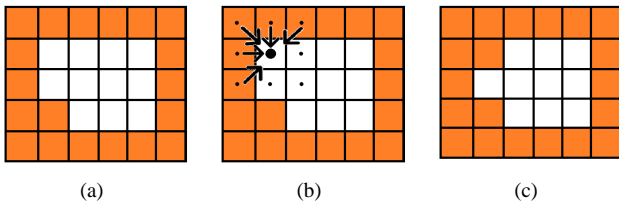
Fig. 5. Example of the diffusion stage of the inpainting algorithm for one pixel: (a) Representation of the initial stage of the diffusion algorithm: pixels under M mask are painted in white whereas pixels outside M are painted in orange; (b) Calculation of the new value from valid neighbors, and (c) Image with new value obtained.
